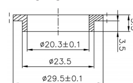
Bearing ring
